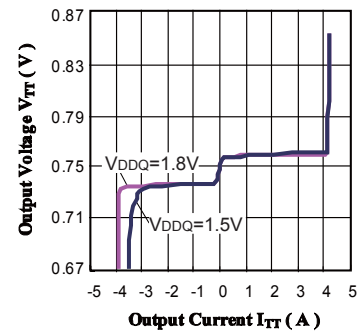
DDR3 Regulation
